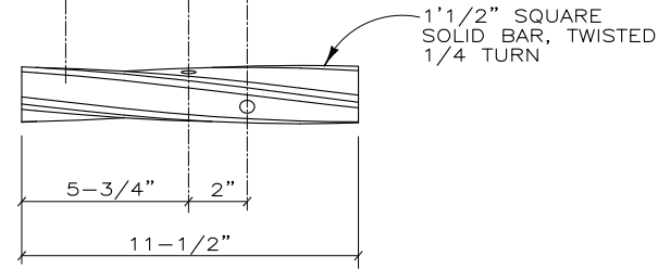
EXTENSION POST 3X SCALE
