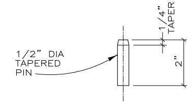
TAPERED PIN 5 X GRAPHIC SCALE
