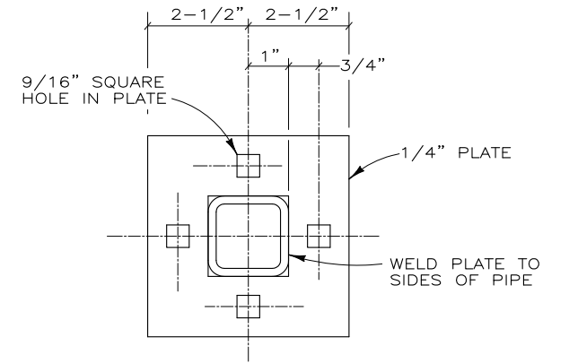
WELDED FLANGE DETAIL 5 X GRAPHIC SCALE
