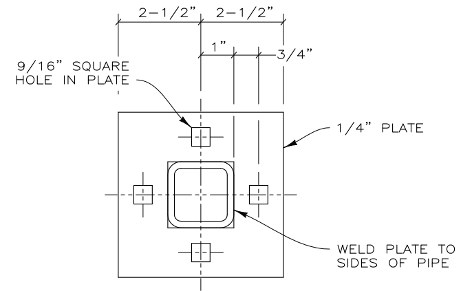
WELDED FLANGE DETAIL NOT TO SCALE
