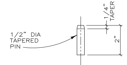
TAPERED PIN NOT TO SCALE
