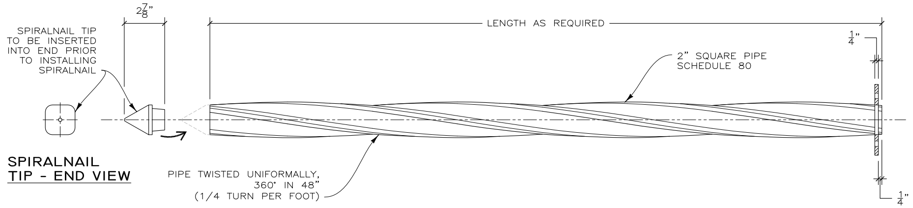
SPIRALNAIL NOT TO SCALE
