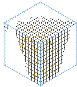
TYPICAL ASSEMBLED GABION NOT TO SCALE
