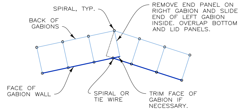
PLAN VIEW CONCAVE ANGLE NOT TO SCALE
