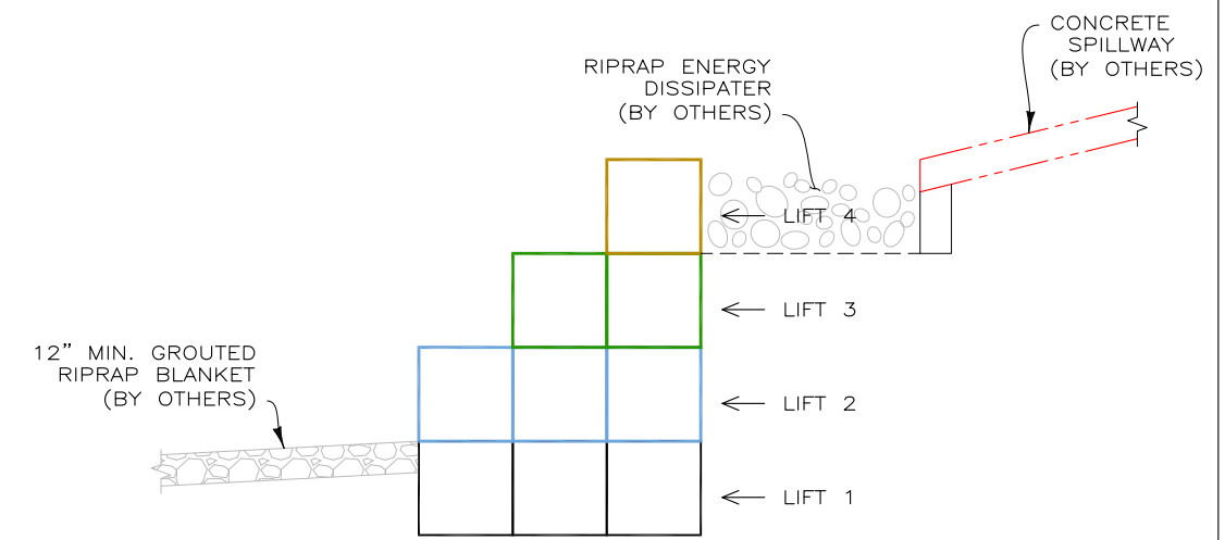
TYPICAL GABION SECTION SCALE: 3" = 20'
