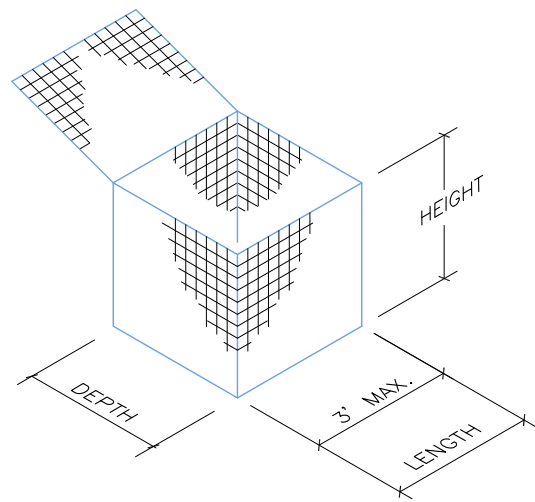
TYPICAL GABION NOT TO SCALE
