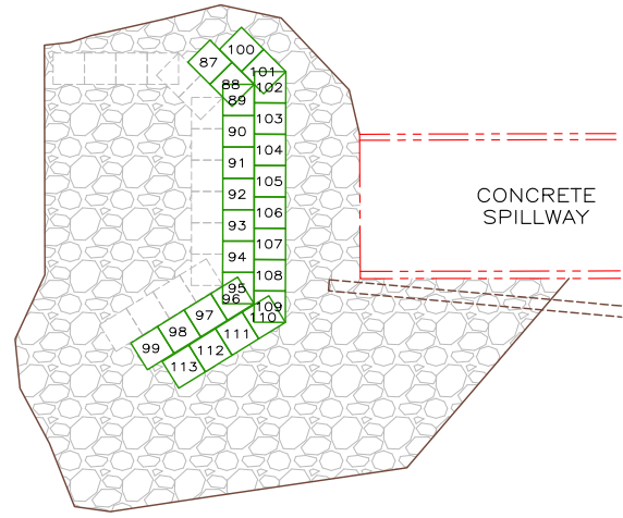
PLAN VIEW - LIFT 3 SCALE: 1" = 20'
