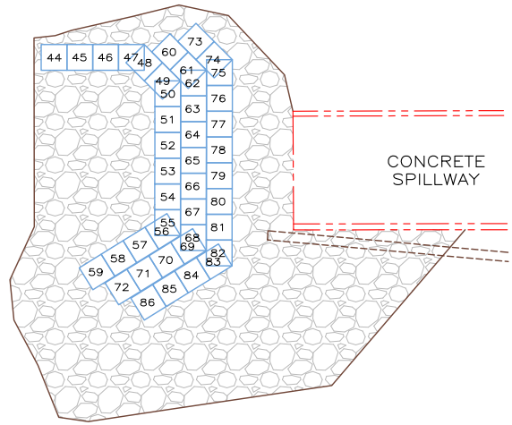
PLAN VIEW - LIFT 2 SCALE: 1" = 20'
