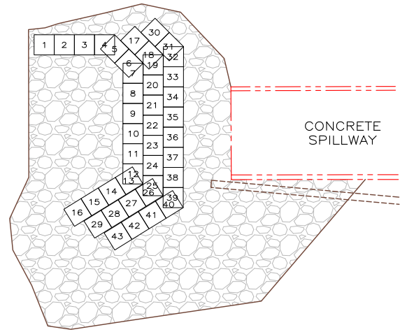
PLAN VIEW - LIFT 1 SCALE: 1" = 20'
