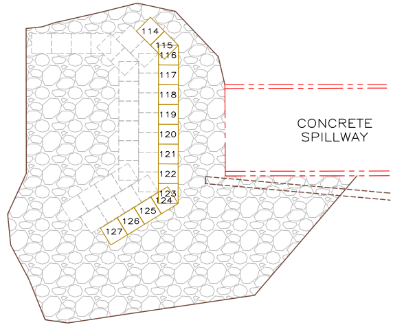
PLAN VIEW - LIFT 4 SCALE: 1" = 20'
