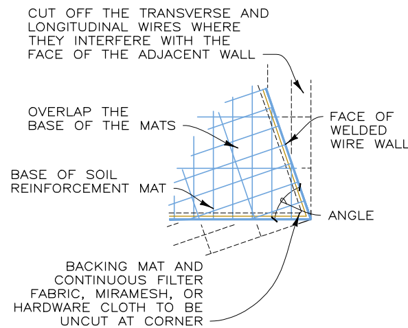
ACUTE CONVEX ANGLE NOT TO SCALE
