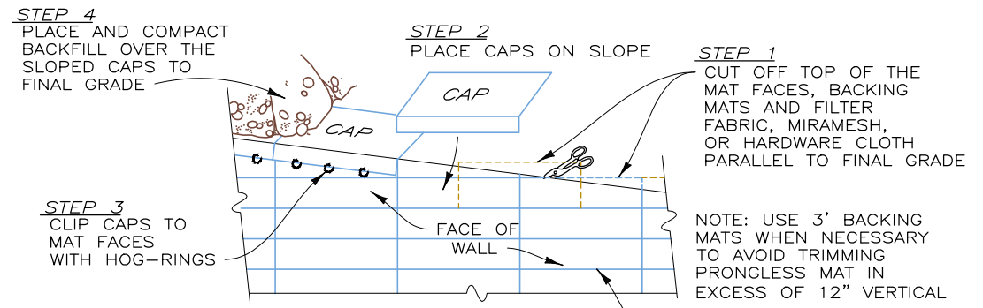
PICTORIAL ELEVATION SLOPED CAP MAT DETAIL NOT TO SCALE
