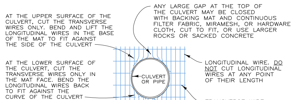
MAT PENETRATION DETAIL NOT TO SCALE
